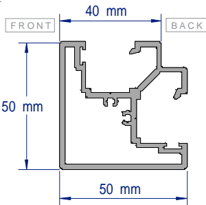
SAP106 50MM CORNER POST 2.8 & 3.6 METRE LENGTHS
