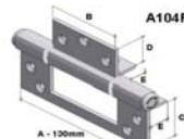
SPAHG104 ALUMINIUM HEAVYDUTY DOUBLE FASTFIX HINGE 130MM X 50MM EACH
