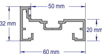
SAP108 45MM DOORFRAME 2.8 & 3.6 METRE LENGTHS
