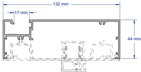
SAP337 FRONT GLAZE FRAME / MULLION COMPLIES WITH AS1428.1 2009 2.8 & 3.6 METRE LENGTHS
