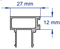
SAPDS35 35MM DOORSTOP
