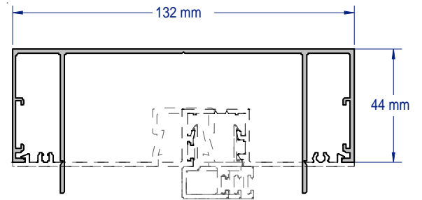
SAP310L 45MM CAPPING HEAD / FRAME COMPLIES WITH AS1428.1 2009 2.8 & 3.6 METRE LENGTHS
