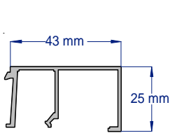
SAP020 25MM SILL BEAD 2.8 & 3.6 METRE LENGTHS
