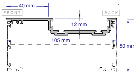
SAP481 SNAP IN CLOSING CHANNEL 2.8 & 3.6 METRE LENGTHS (MUST BE USED IN CONJUNCTION WITH MICROLINE ONLY FOR FRONT FRAMING)
