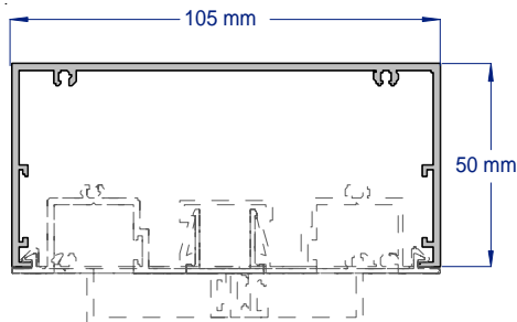
SAP012L 50MM CAPPING HEAD / WALLSTARTER COMPLIES WITH AS1428.1 2009 2.8 & 3.6 METRE LENGTHS
