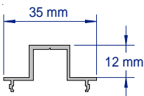
SAP111C SHADOWLINE SNAPIN 2.8 & 3.6 METRE LENGTHS
