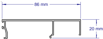
SAP239 FRONT GLAZE SILL BEAD 2.8 & 3.6 METRE LENGTHS
