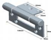
SPAHG105 ALUMINIUM HEAVYDUTY SINGLE FASTFIX HINGE 130MM X 50MM EACH
