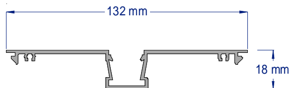
SAP316 SNAP IN POCKET GLAZE 2.8 & 3.6 METRE LENGTHS
