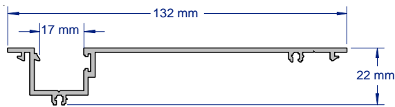
SAP338 FRONT GLAZE SNAPIN 2.8 & 3.6 METRE LENGTHS
