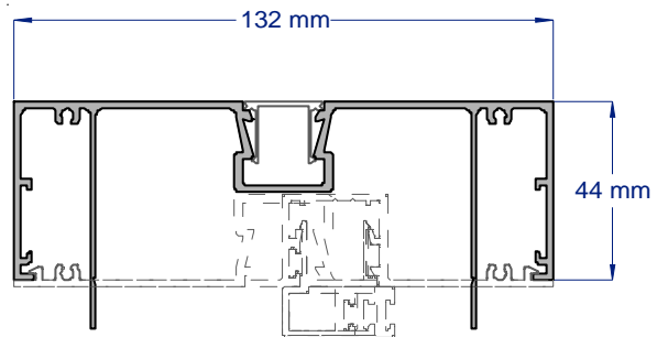
SAP314L 45MM PLASTERBOARD POCKET FIN FRAME COMPLIES WITH AS1428.1 2009 2.8 & 3.6 METRE LENGTHS
