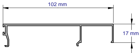
SAP339 FRONT GLAZE SILL BEAD 2.8 & 3.6 METRE LENGTHS
