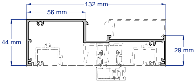
SAP319L 45MM SILL/TRANSOM COMPLIES WITH AS1428.1 2009 2.8 & 3.6 METRE LENGTHS
