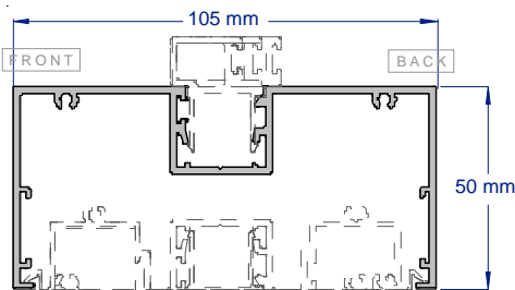
SAP012L 50MM CAPPING HEAD / WALLSTARTER COMPLIES WITH AS1428.1 2009 2.8 & 3.6 METRE LENGTHS
