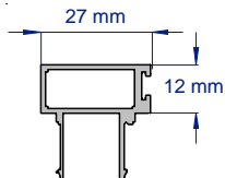
SAPDS35 35MM DOORSTOP (NEW)
