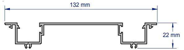
SAP341 DOUBLE GLAZE SNAPIN 2.8 & 3.6 METRE LENGTHS
