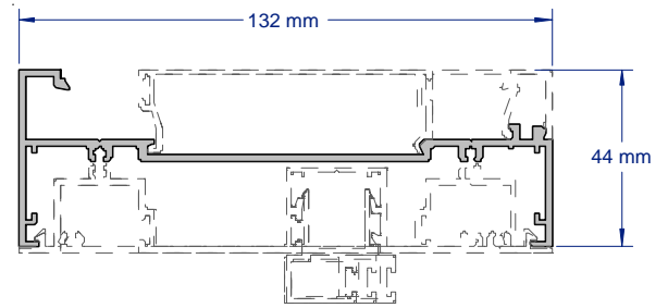
SAP340 FRONT & DOUBLE GLAZE SILL / MULLION / TRANSOM COMPLIES WITH AS1428.1 2009 2.8 & 3.6 METRE LENGTHS
