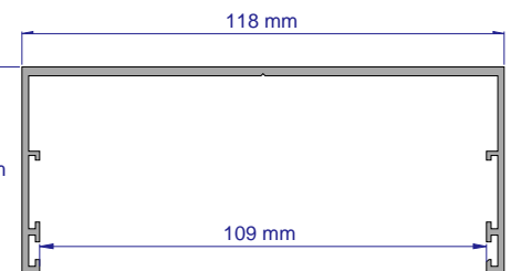
SAPWSH SUB HEAD - DEFLECTION 3.6 METRE LENGTHS (MUST BE USED IN CONJUNCTION WITH WIDELINE & FRONTLINE FRAMING)
