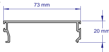
SAP343 DOUBLE GLAZE CAP 2.8 & 3.6 METRE LENGTHS
