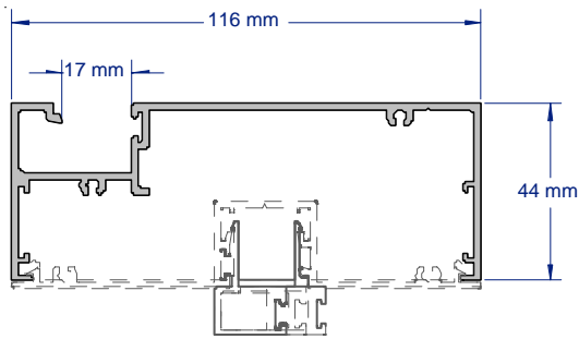
SAP237 FRONT GLAZE FRAME / MULLION COMPLIES WITH AS1428.1 2009 2.8 & 3.6 METRE LENGTHS
