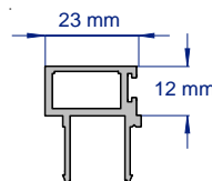
SAPDS40 40MM DOORSTOP (NEW)
