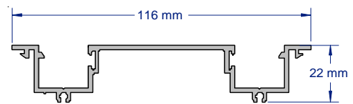
SAP241 DOUBLE GLAZE SNAPIN 2.8 & 3.6 METRE LENGTHS
