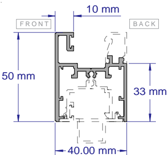
SAP119 50MM TRANSOM/SILL NEW VERSION 2.8 & 3.6 METRE LENGTHS
