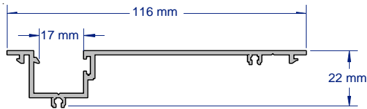
SAP238 FRONT GLAZE SNAPIN 2.8 & 3.6 METRE LENGTHS
