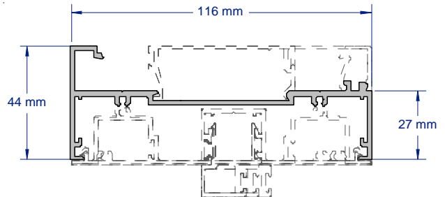
SAP240 DOUBLE GLAZE SILL / MULLION / TRANSOM COMPLIES WITH AS1428.1 2009 2.8 & 3.6 METRE LENGTHS
