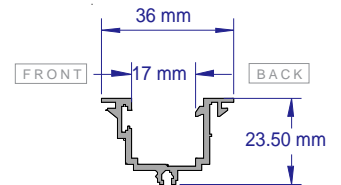
SAP116 GLAZING INFILL 2.8 & 3.6 METRE LENGTHS
