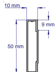
SAP116 GLAZING INFILL 2.8 & 3.6 METRE LENGTHS
