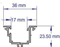
SAP116 MIDRAIL ADAPTOR FOR SAP526 2.8 & 3.6 METRE LENGTHS
