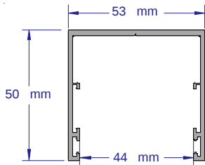
SAPMSH SUB HEAD - DEFLECTION 3.6 METRE LENGTHS
