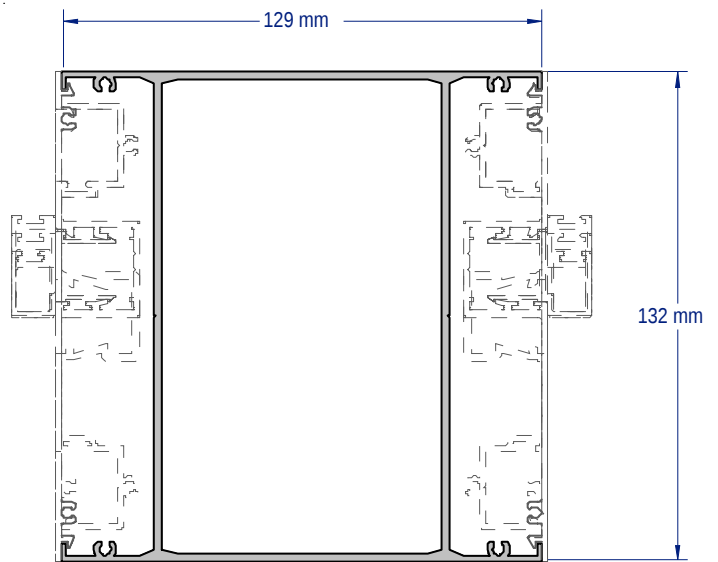
SAP324D 132MM 2 WAY POST COMPLIES WITH AS1428.1 2009 2.8 & 3.6 METRE LENGTHS
