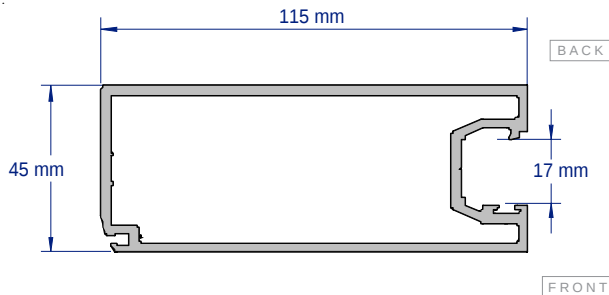
SAP521 115MM WIDE LOCK STILE 2.8 & 3.6 METRE LENGTHS
