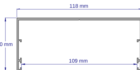
SAPWSH SUB HEAD - DEFLECTION 3.6 METRE LENGTHS (MUST BE USED IN CONJUNCTION WITH WIDELINE & FRONTLINE FRAMING)
