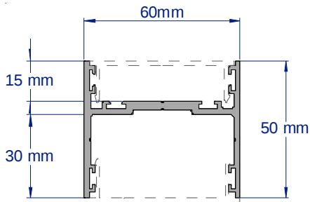
SAP582 50MM OVERHEAD/CLOSING CHANNEL 2.8, 3.6 & 5.6 METRE LENGTHS
