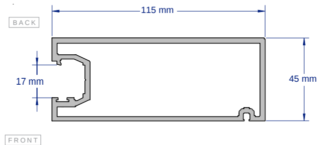
SAP520 115MM WIDE SLIDER STILE 2.8 & 3.6 METRE LENGTHS
