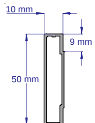
SAP116 GLAZING INFIL 2.8 & 3.6 METRE LENGTHS
