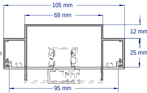
SAP010C 25MM SHADOWLINE CAPPING HEAD / FRAME 2.8 & 3.6 METRE LENGTHS
