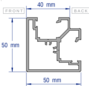
SAP106 50MM CORNER POST 2.8 & 3.6 METRE LENGTHS
