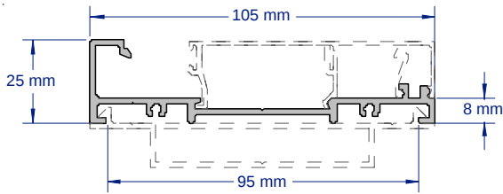
SAP033 25MM FRONT/DOUBLE GLAZING SILL 2.8 & 3.6 METRE LENGTHS
