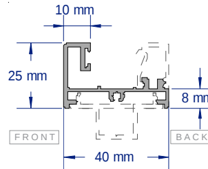
SAP104 GLAZING SILL 2.8 & 3.6 METRE LENGTHS
