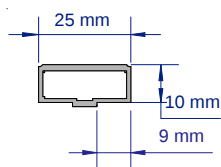
SAP25T 25MM STICK ON MULLION / TRANSOM TRIM 2.8 & 3.6 METRE LENGTHS
