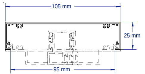
SAP012 25MM CAPPING HEAD / WALLSTARTER 2.8 & 3.6 METRE LENGTHS
