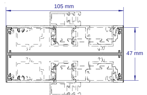
SAP021 50MM MULTICAP COMPLIES WITH AS1428.1 2009 2.8 & 3.6 METRE LENGTHS (NEW)
