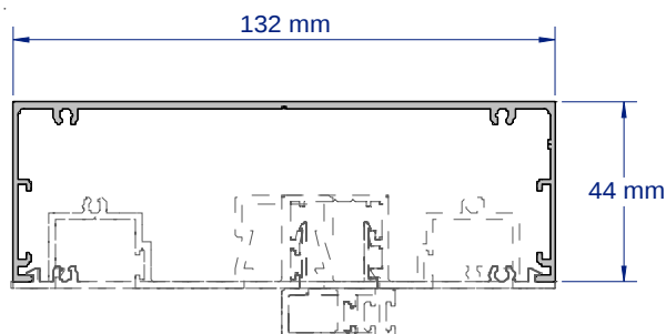
SAP312L 45MM CAPPING / WALLSTARTER COMPLIES WITH AS1428.1 2009 2.8 & 3.6 METRE LENGTHS
