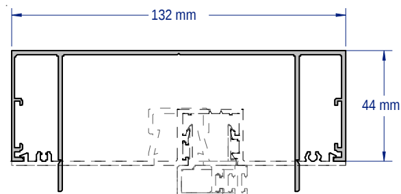
SAP310L 45MM CAPPING HEAD / FRAME COMPLIES WITH AS1428.1 2009 2.8 & 3.6 METRE LENGTHS
