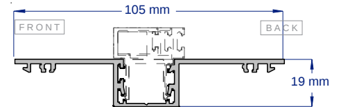
SAP016 SNAP IN POCKET GLAZE 2.8 & 3.6 METRE LENGTHS
