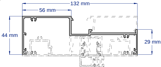
SAP319L 45MM SILL/TRANSOM COMPLIES WITH AS1428.1 2009 2.8 & 3.6 METRE LENGTHS
