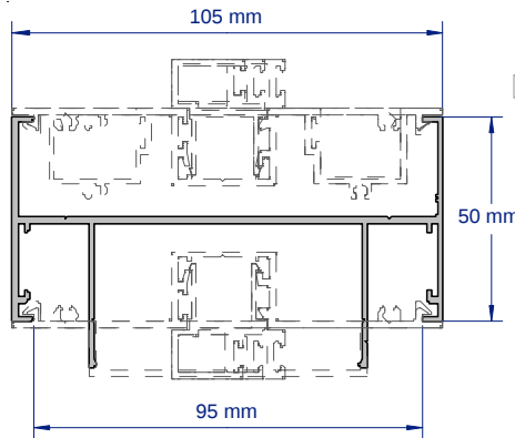
SAP013L 50MM CAPPING HEAD / FRAME COMPLIES WITH AS1428.1 2009 2.8 & 3.6 METRE LENGTHS
