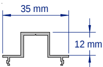
SAP111C SHADOWLINE SNAPIN 2.8 & 3.6 METRE LENGTHS
