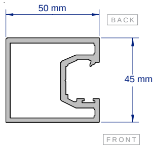
SAP510 50MM PLAIN STILE 2.8 & 3.6 METRE LENGTHS
