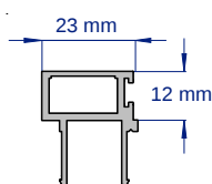
SAPDS40 40MM DOORSTOP
