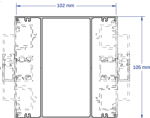
SAP024D 2 WAY POST COMPLIES WITH AS1428.1 2009 2.8 & 3.6 METRE LENGTHS
