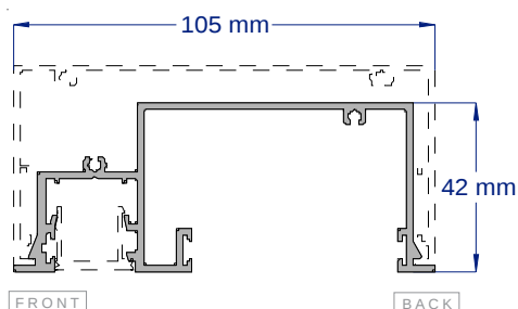
SAP480 SNAP IN GLAZING SLIDE HEAD CHANNEL 2.8 & 3.6 METRE LENGTHS (MUST BE USED IN CONJUNCTION WITH MICROLINE ONLY FOR FRONT FRAMING)
