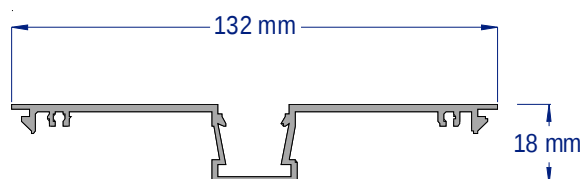
SAP316 SNAP IN POCKET GLAZE 2.8 & 3.6 METRE LENGTHS
