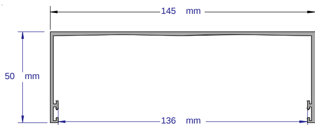
SAP3SH 92MM MAXLINE SUB HEAD - DEFLECTION 2.8 & 3.6 METRE LENGTHS
