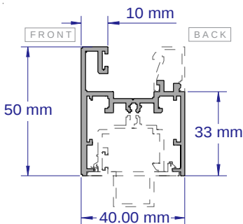
SAP119 50MM TRANSOM/SILL 2.8 & 3.6 METRE LENGTHS NEW VERSION
