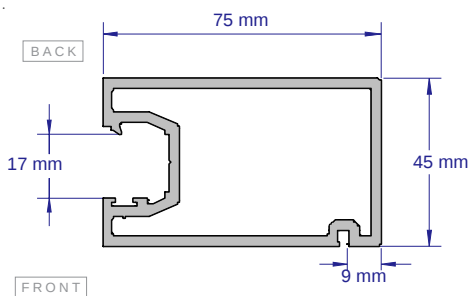
SAP523 75MM SLIDE STILE 2.8 & 3.6 METRE LENGTHS
