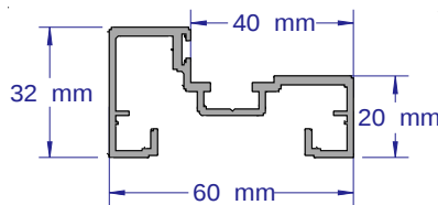
SAP107 35MM DOORFRAME 2.8 & 3.6 METRE LENGTHS
