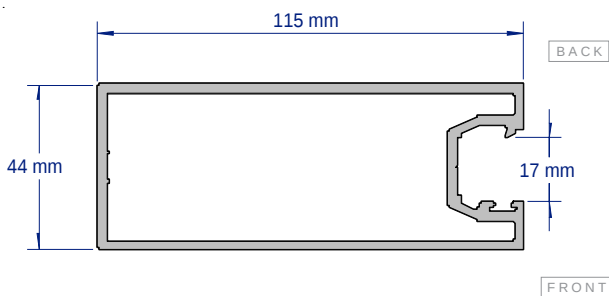
SAP519 115MM WIDE PLAIN STILE (LOCK/HINGE) 2.8 & 3.6 METRE LENGTHS
