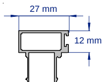
SAPDS35 35MM DOORSTOP
