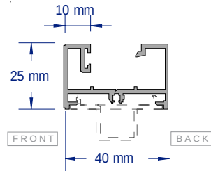
SAP103 GLAZING FRAME 2.8 & 3.6 METRE LENGTHS
