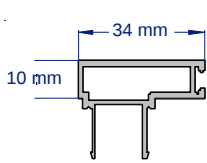
SAP317 35MM DOORSTOP 2.8 & 3.6 METRE LENGTHS
