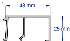
SAP020 25MM SILL BEAD 2.8 & 3.6 METRE LENGTHS
