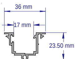
SAP116 MIDRAIL ADAPTOR FOR SAP526 2.8 & 3.6 METRE LENGTHS
