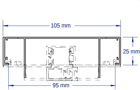
SAP010 25MM CAPPING HEAD / FRAME 2.8 & 3.6 METRE LENGTHS
