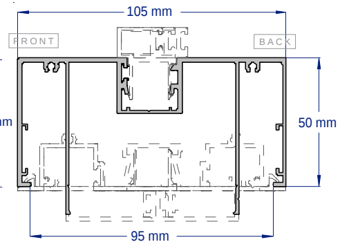
SAP014F 50MM PLASTERBOARD POCKET FRAME COMPLIES WITH AS1428.1 2009 2.8 & 3.6 METRE LENGTHS
