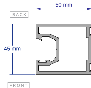
SAP511 50MM CLOSING STILE 2.8 & 3.6 METRE LENGTHS
