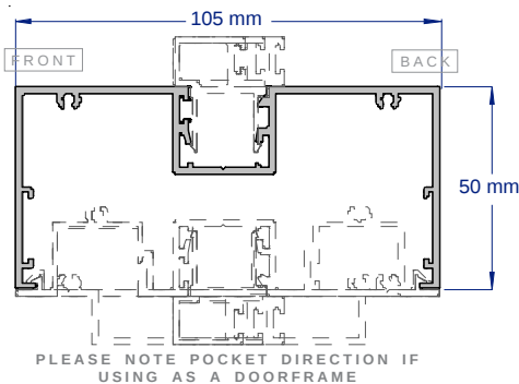
SAP014L 50MM POCKET CAPPING / FRAME COMPLIES WITH AS1428.1 2009 2.8 & 3.6 METRE LENGTHS
