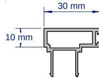
SAP318B 40MM DOORSTOP 2.8 & 3.6 METRE LENGTHS
