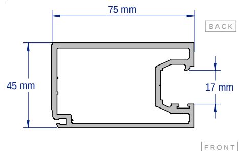
SAP522 75MM LOCK STILE 2.8 & 3.6 METRE LENGTHS
