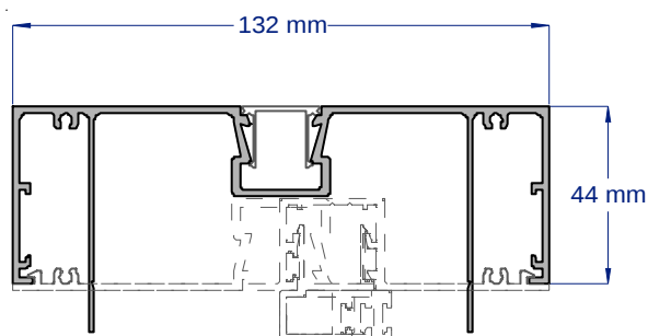
SAP314L 45MM PLASTERBOARD POCKET FIN FRAME COMPLIES WITH AS1428.1 2009 2.8 & 3.6 METRE LENGTHS
