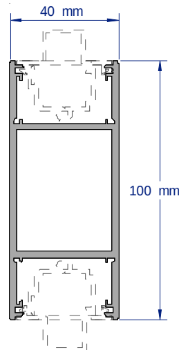
SAP114 100MM MULTICAP/TRANSOM 2.8 & 3.6 METRE LENGTHS
