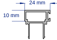
SAP318 45MM DOORSTOP 2.8 & 3.6 METRE LENGTHS
