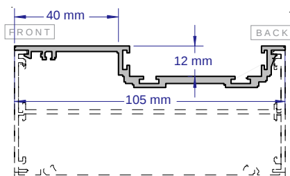
SAP481 SNAP IN CLOSING CHANNEL 2.8 & 3.6 METRE LENGTHS (MUST BE USED IN CONJUNCTION WITH MICROLINE ONLY FOR FRONT FRAMING)
