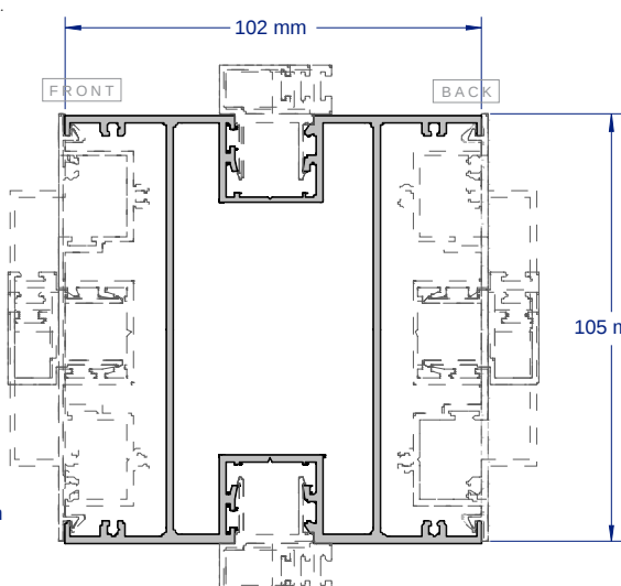
SAP024 4 WAY CORNER POST COMPLIES WITH AS1428.1 2009 2.8 & 3.6 METRE LENGTHS
