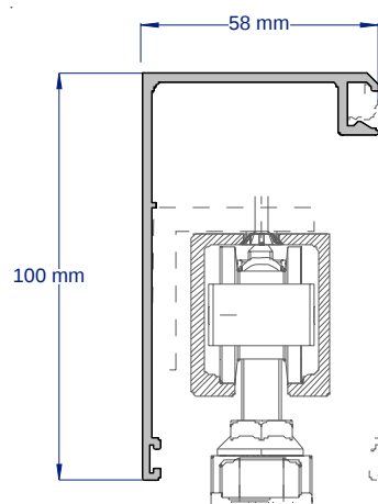
SAP585 SHOOSHLINE OVERHEAD PELMET 3.6 METRE LENGTHS (DOOR TRACK & FIXING ANGLE SOLD SEPERATELY)
