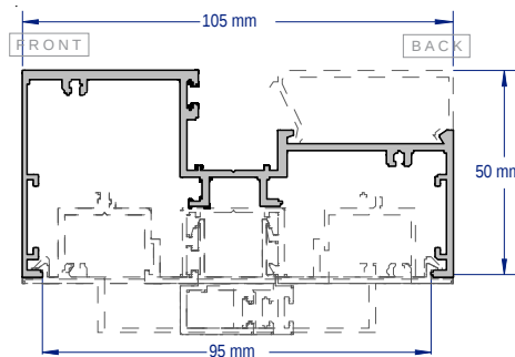
SAP019L 50MM SILL/TRANSOM 2.8 & 3.6 METRE LENGTHS
