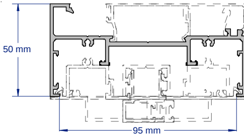
SAP040 50MM FRONT/DOUBLE GLAZE SILL/TRANSOM COMPLIES WITH AS1428.1 2009 2.8 & 3.6 METRE LENGTHS
