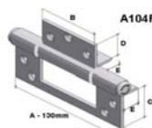
SPAHG104 ALUMINIUM HEAVYDUTY DOUBLE FASTFIX HINGE 130MM X 50MM EACH
