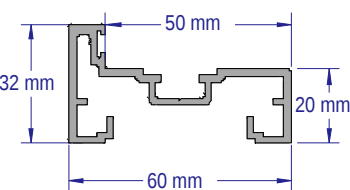
SAP108 45MM DOORFRAME 2.8 & 3.6 METRE LENGTHS
