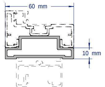
SAP109 ELECTRIC STRIKE ADAPTOR 2.8 & 3.6 METRE LENGTHS
