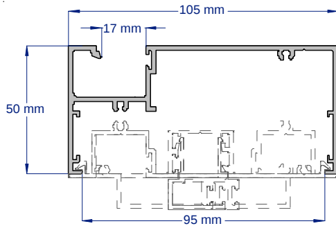
SAP037 50MM GLAZING FRAME/MULLION COMPLIES WITH AS1428.1 2009 2.8 & 3.6 METRE LENGTHS
