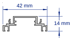
SAP535 CLIP IN BOTTOM SEAL ROLLER GUIDE FOR SAP525/526 3.6 METRE LENGTHS (TOP BE NOTCHED WITH SAW WHERE SCREWS FOR SPIGGOT ARE LOCATED WHEN USING WITH SAP525)
