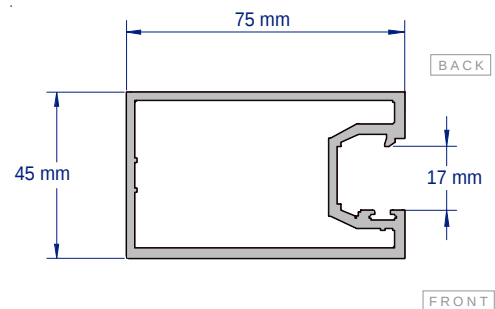
SAP524 75MM PLAIN STILE (LOCK/HINGE) 2.8 & 3.6 METRE LENGTHS
