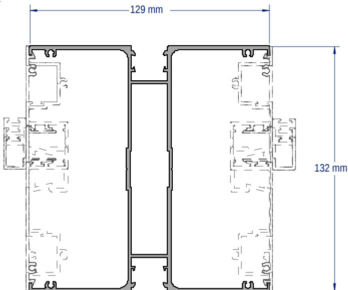
SAP324 132MM 4 WAY POST COMPLIES WITH AS1428.1 2009 2.8 & 3.6 METRE LENGTHS
